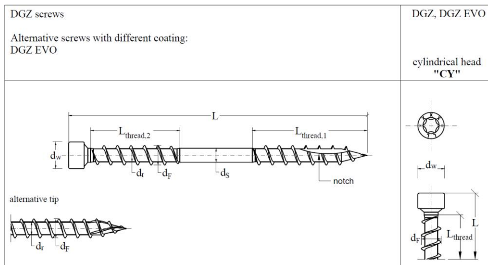
FIGURE 4—DGZ AND DGZ EVO DOUBLE THREADED SCREWS
