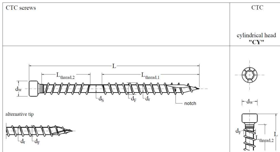
FIGURE 5—CTC DOUBLE THREADED SCREWS
