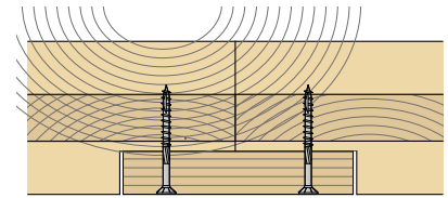
SPLINE JOINT
