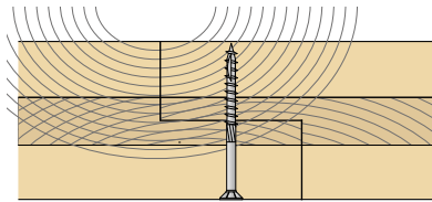
HALF-LAP JOINT
