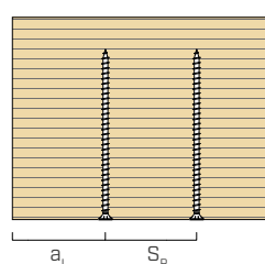
façade
