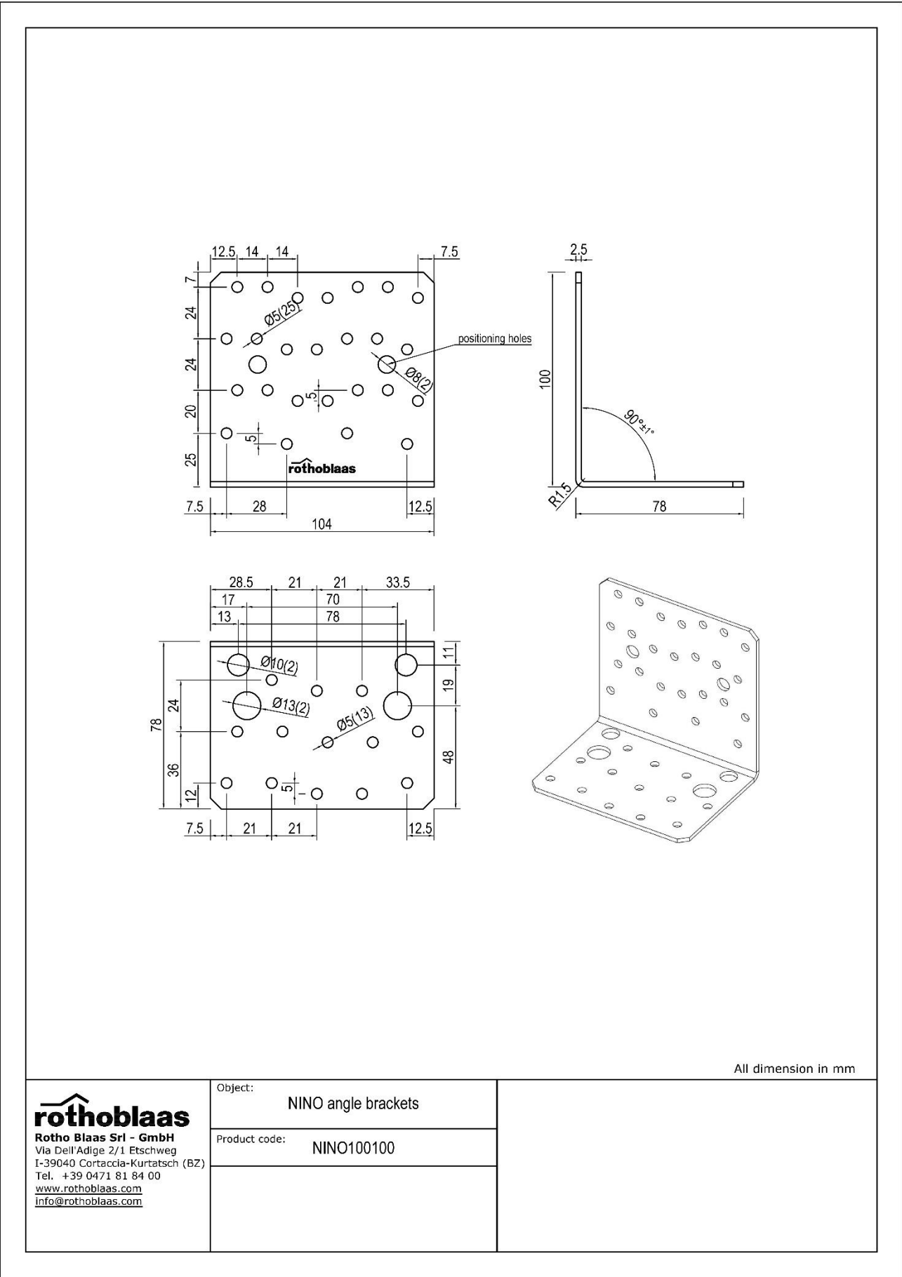
Figure B. 1 Dimensions of Angle Bracket NINO 100100
