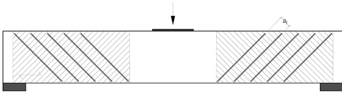
Figure E.1: Timber member with shear reinforcement; shaded areas: reinforced areas with screws arranged under 45°
