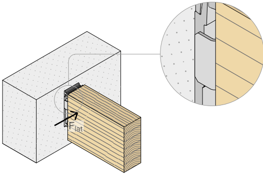
LOCK STOP
