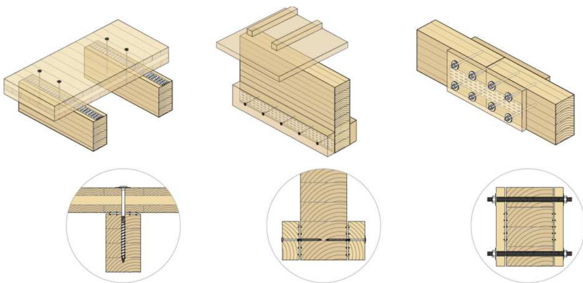
Figure A2.3: Examples for typical applications of SHARP METAL in mechanically jointed beams
